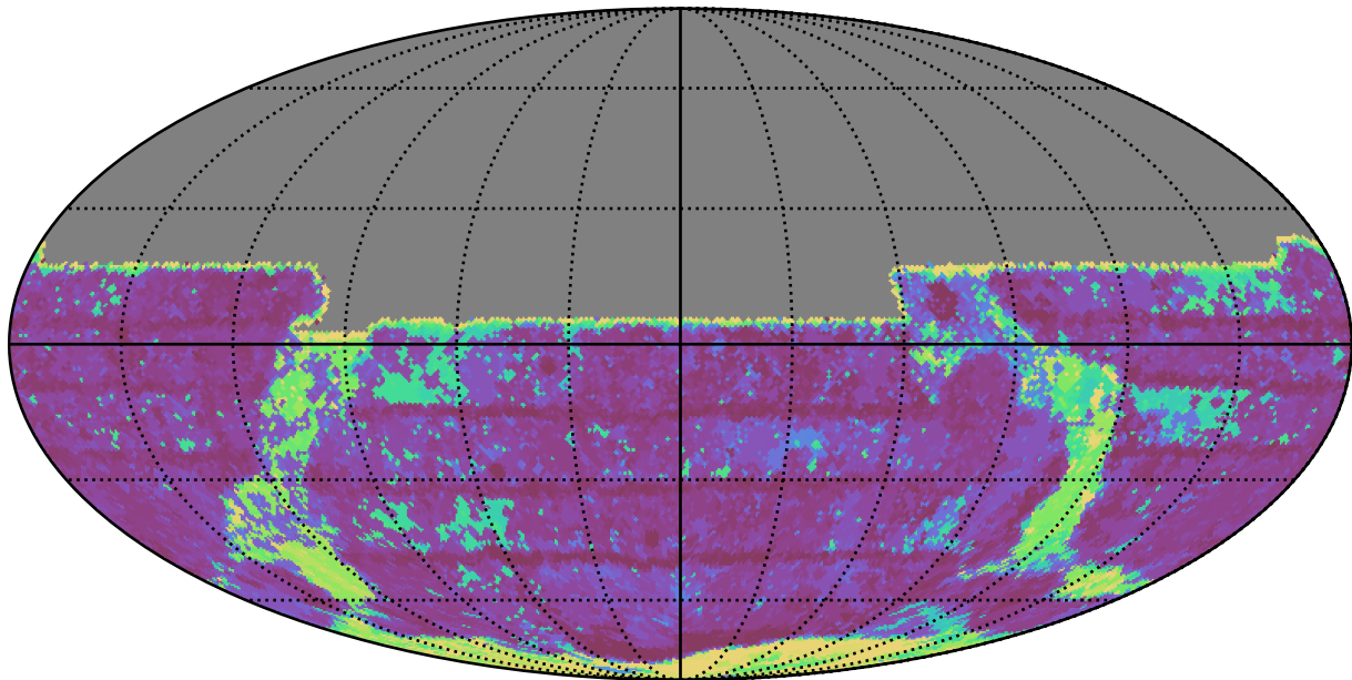
ddf_loaded_fl2_v3.4_10yrs All sky y band: Max Inter-Night Gap
