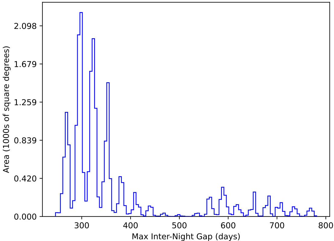
ddf_loaded_fl2_v3.4_10yrs All sky y band: Max Inter-Night Gap
