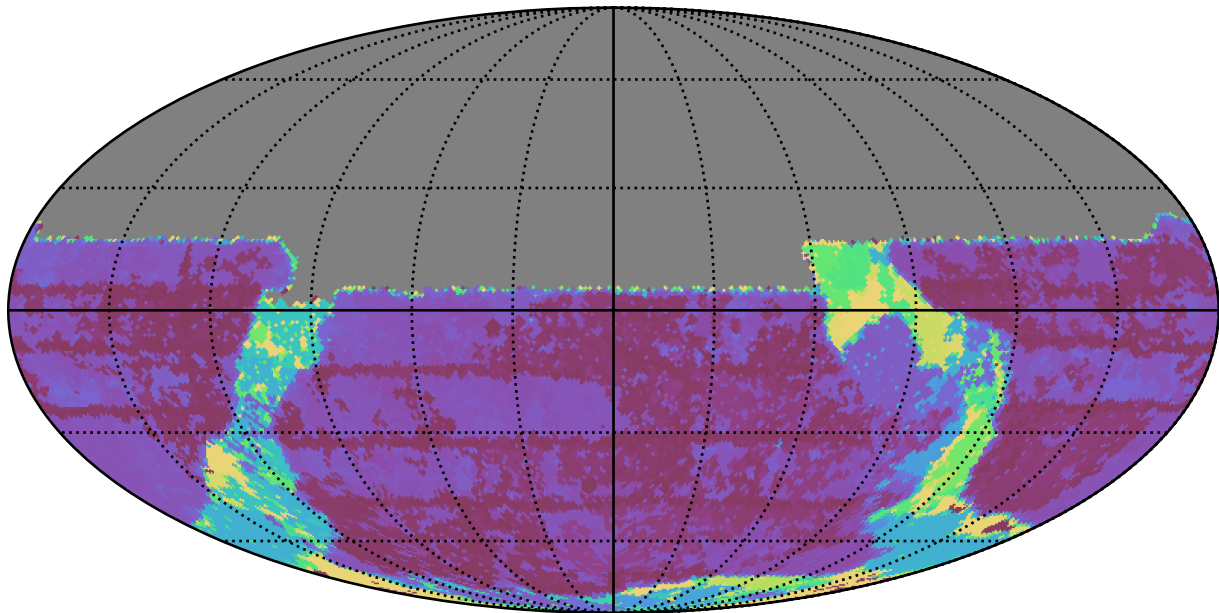
ddf_loaded_fl2_v3.4_10yrs All sky u band: Max Inter-Night Gap
