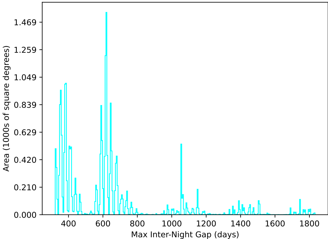
ddf_loaded_fl2_v3.4_10yrs All sky u band: Max Inter-Night Gap
