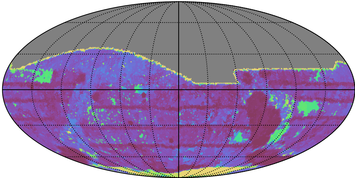
ddf_loaded_fl2_v3.4_10yrs All sky r band: Max Inter-Night Gap
