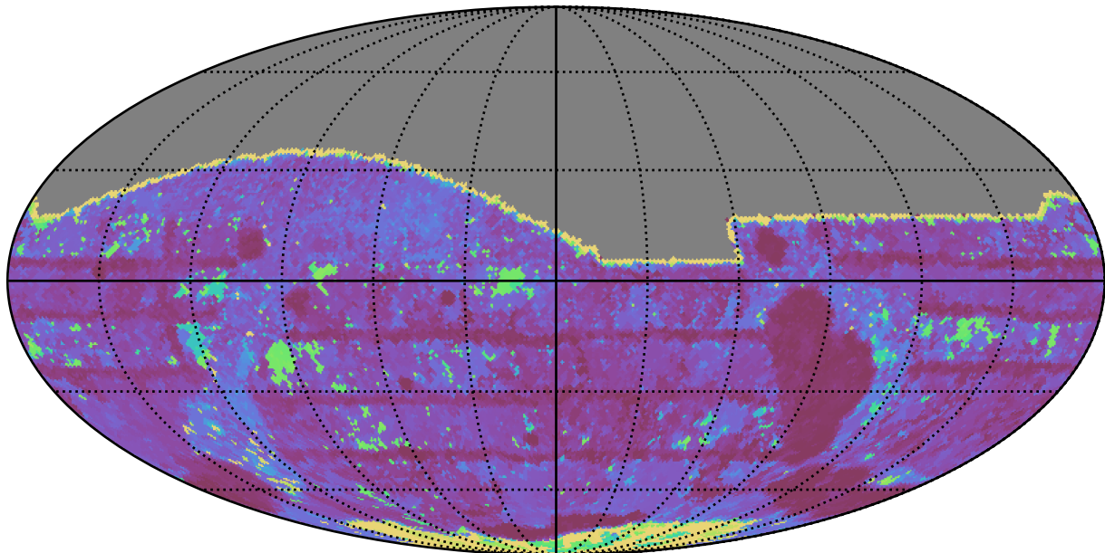
ddf_loaded_fl2_v3.4_10yrs All sky i band: Max Inter-Night Gap
