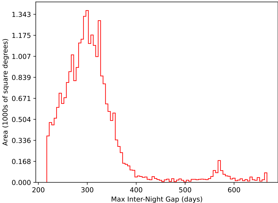
ddf_loaded_fl2_v3.4_10yrs All sky i band: Max Inter-Night Gap
