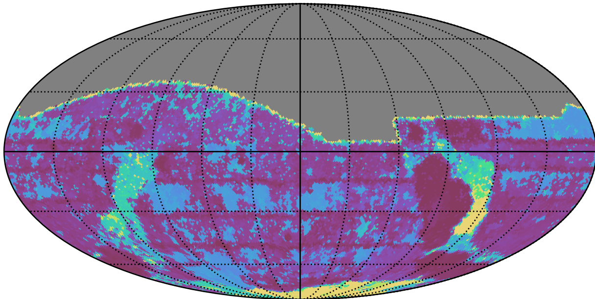
ddf_loaded_fl2_v3.4_10yrs All sky g band: Max Inter-Night Gap
