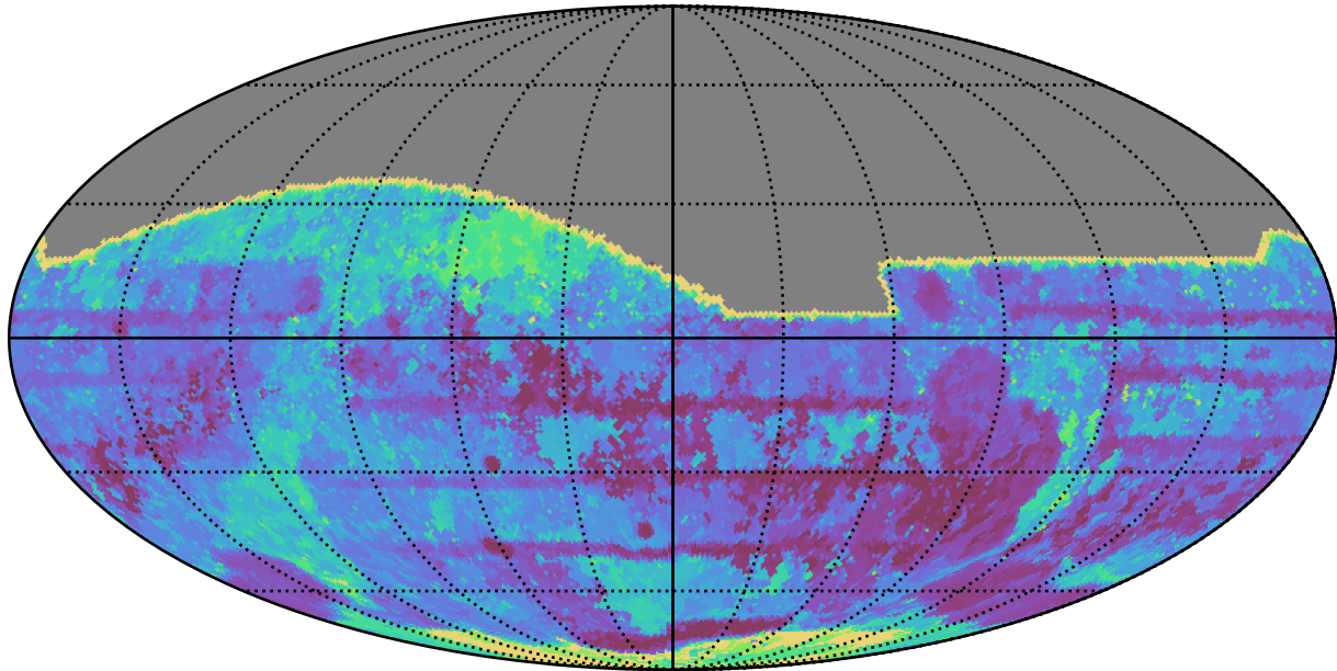
ddf_loaded_fl2_v3.4_10yrs All sky all bands: Max Inter-Night Gap
