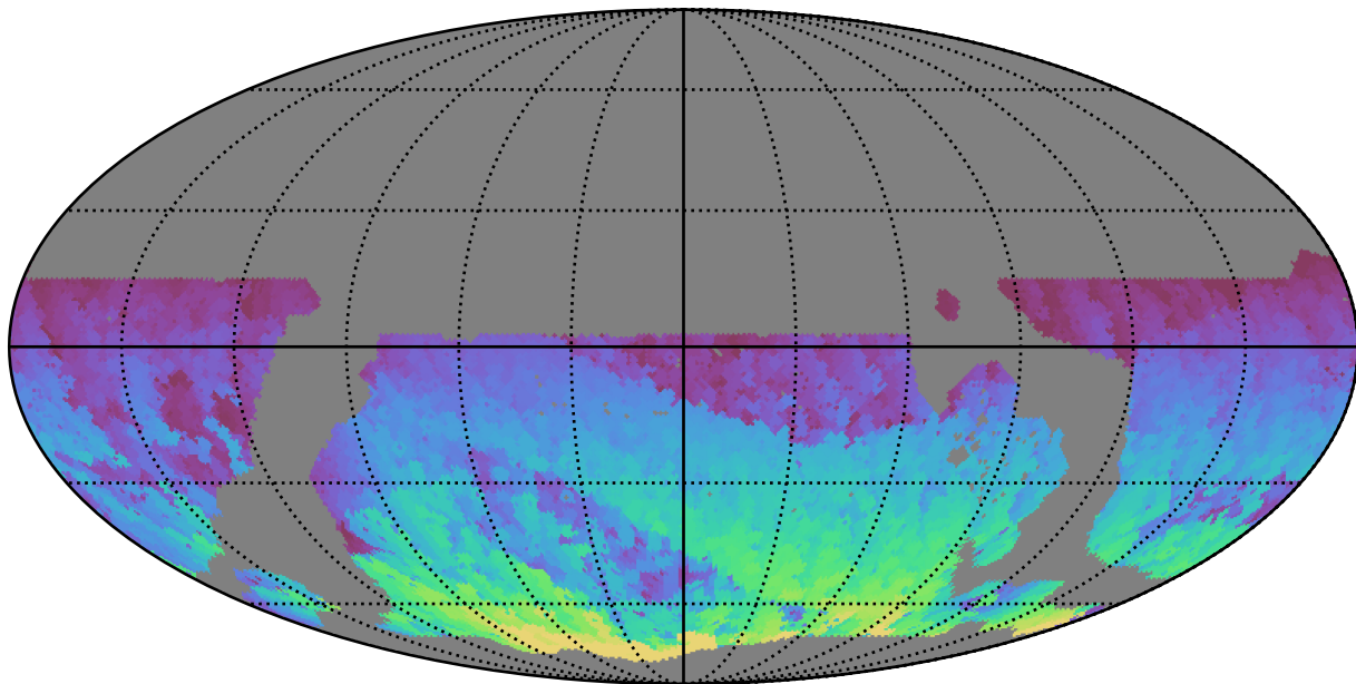
ddf_loaded_fl2_v3.4_10yrs WFD z band: Max HA
