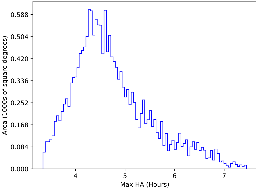
ddf_loaded_fl2_v3.4_10yrs WFD y band: Max HA
