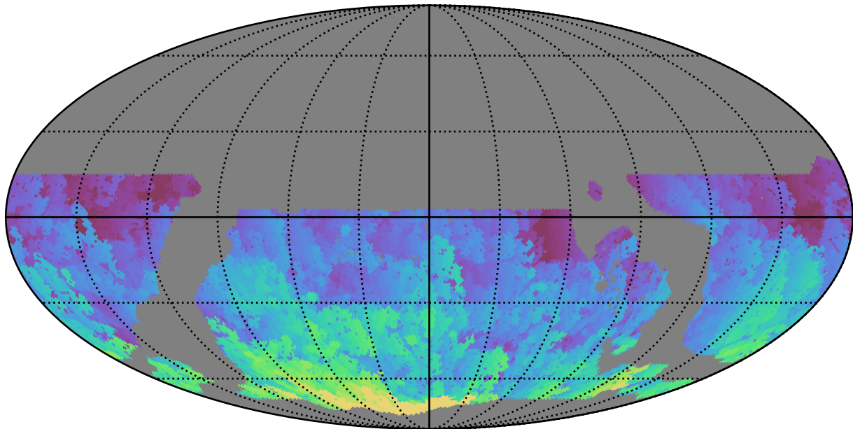
ddf_loaded_fl2_v3.4_10yrs WFD u band: Max HA
