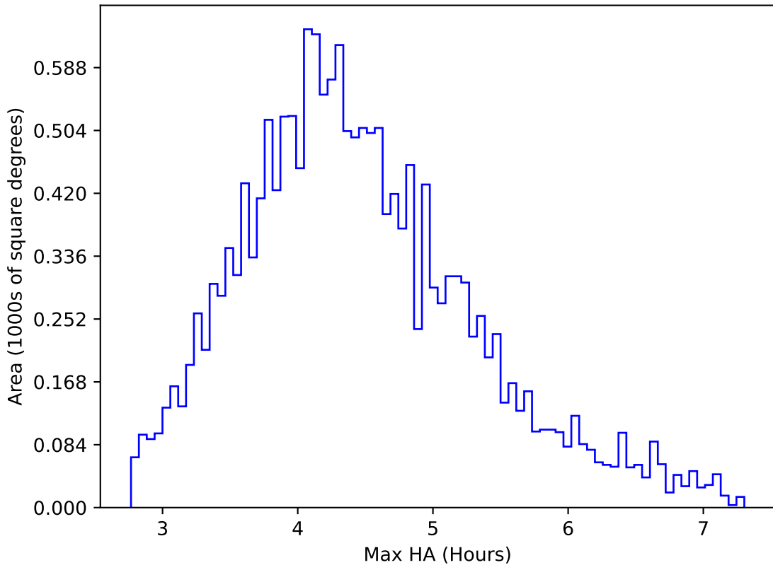
ddf_loaded_fl2_v3.4_10yrs WFD r band: Max HA
