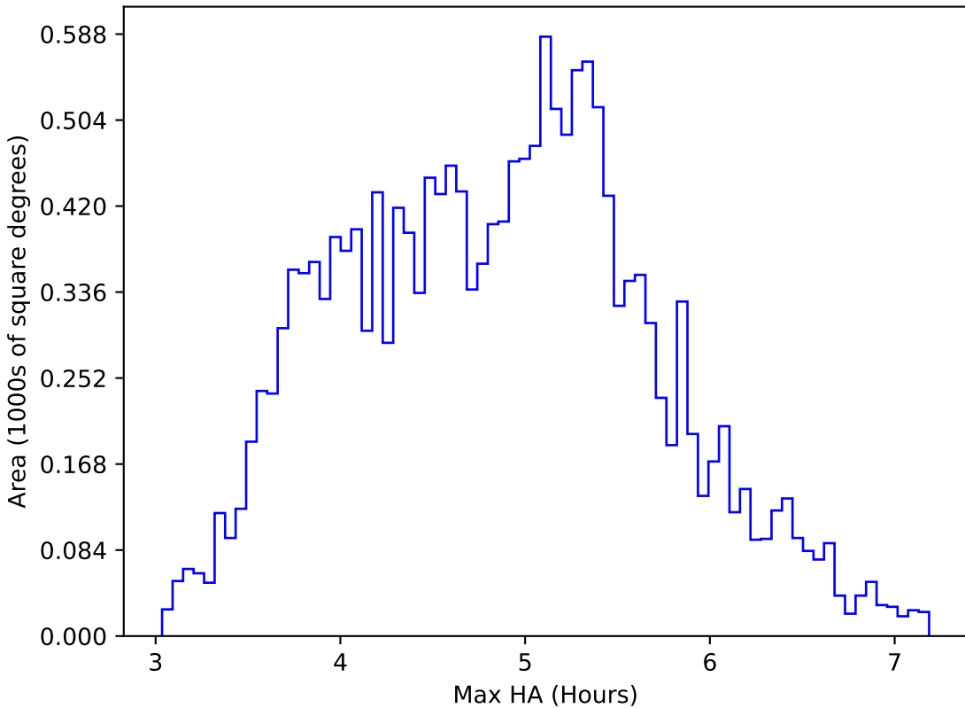
ddf_loaded_fl2_v3.4_10yrs WFD i band: Max HA
