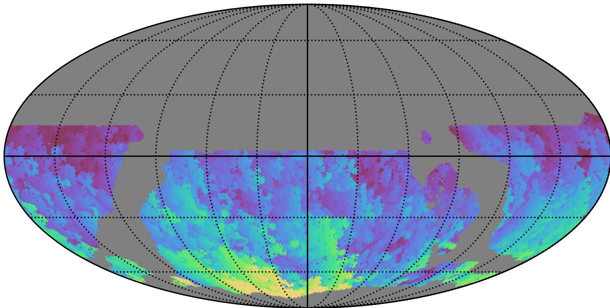
ddf_loaded_fl2_v3.4_10yrs WFD g band: Max HA
