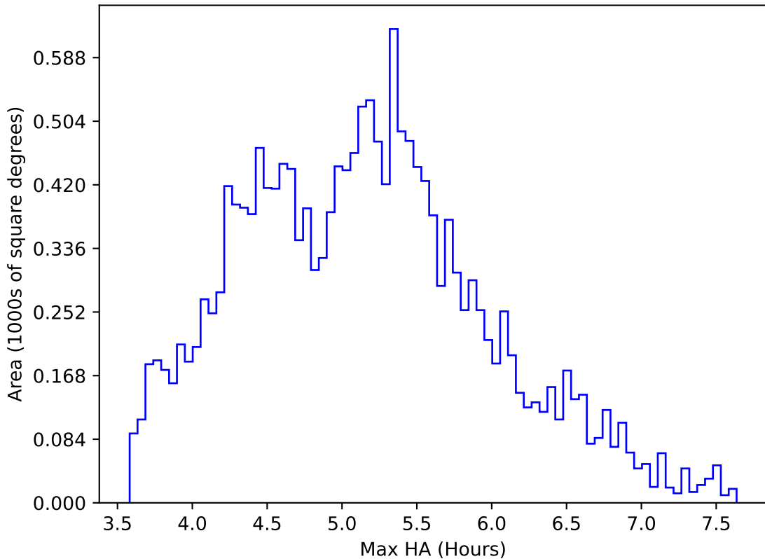
ddf_loaded_fl2_v3.4_10yrs WFD all bands: Max HA
