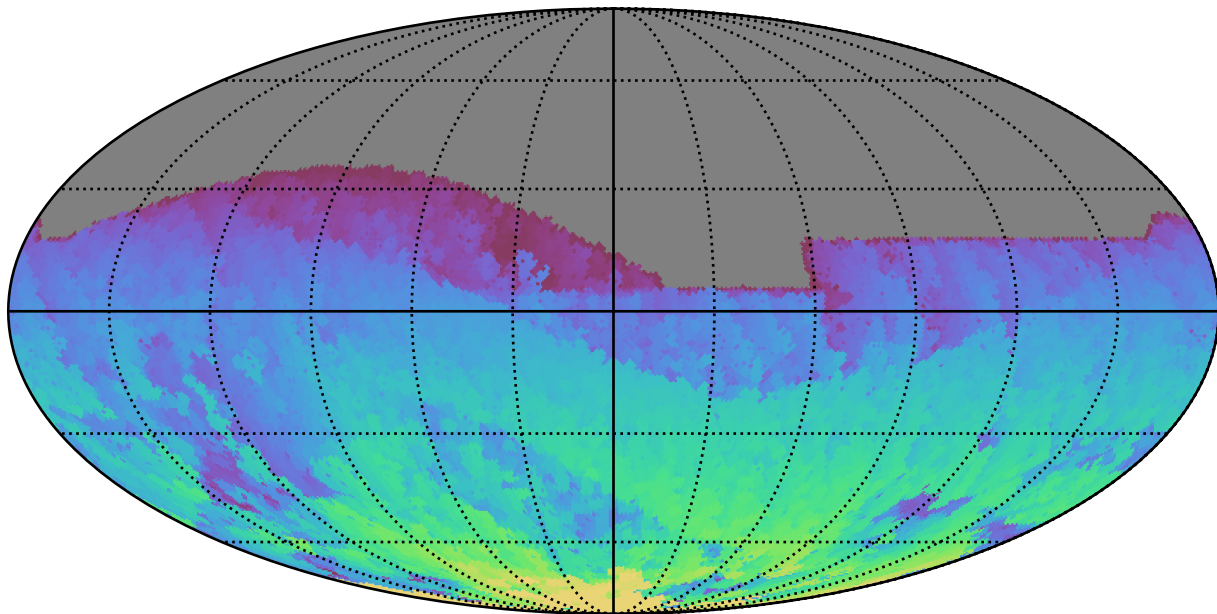
ddf_loaded_fl2_v3.4_10yrs All sky z band: Max HA
