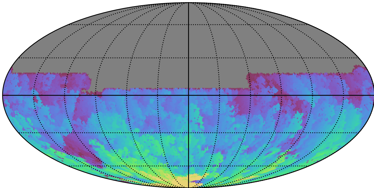
ddf_loaded_fl2_v3.4_10yrs All sky u band: Max HA
