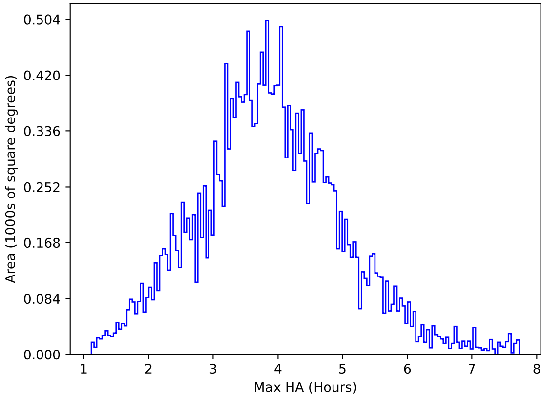
ddf_loaded_fl2_v3.4_10yrs All sky u band: Max HA
