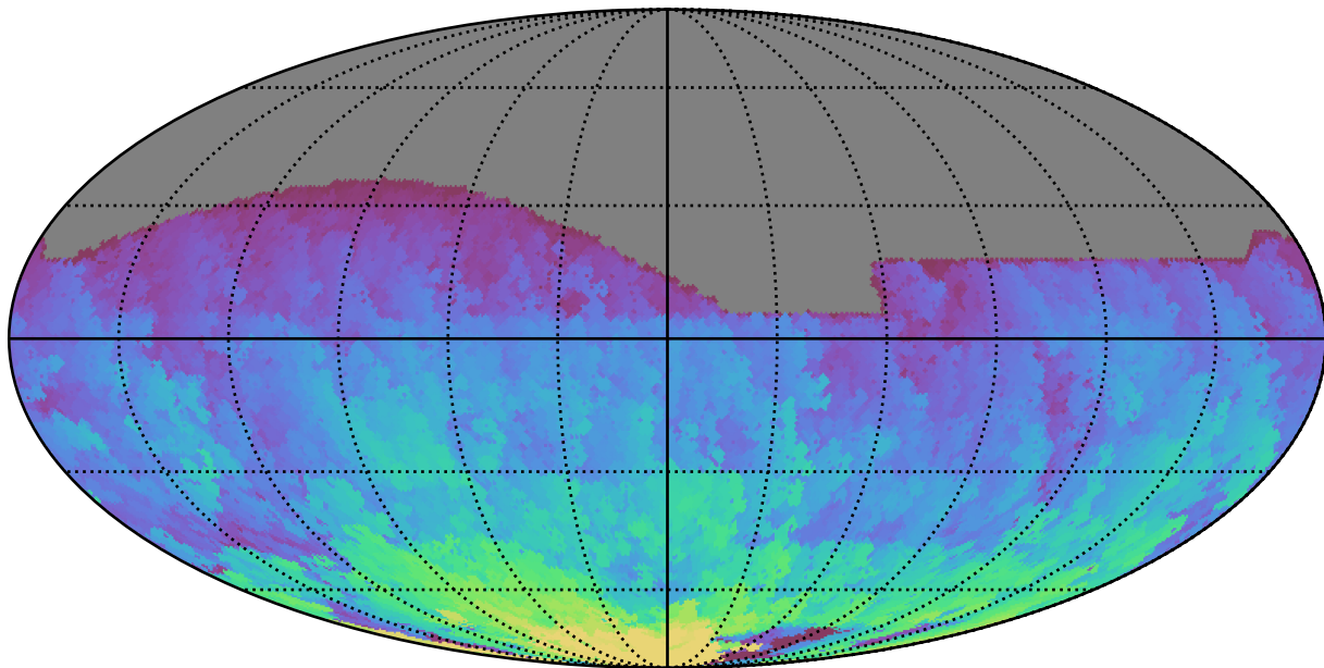
ddf_loaded_fl2_v3.4_10yrs All sky r band: Max HA
