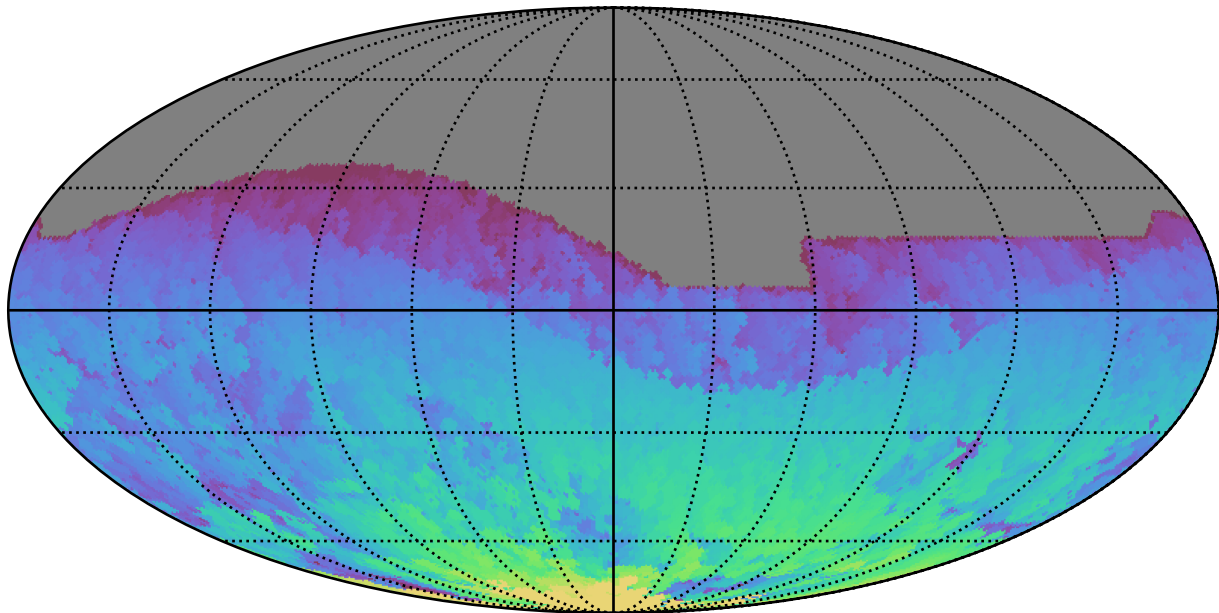
ddf_loaded_fl2_v3.4_10yrs All sky i band: Max HA
