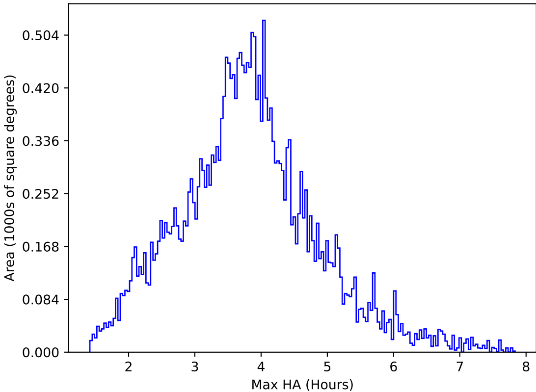
ddf_loaded_fl2_v3.4_10yrs All sky g band: Max HA
