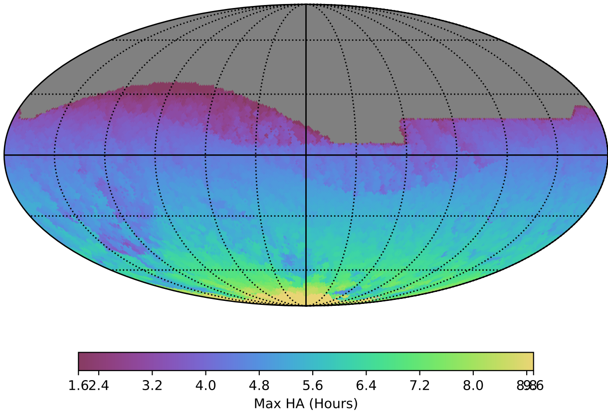
ddf_loaded_fl2_v3.4_10yrs All sky all bands: Max HA
