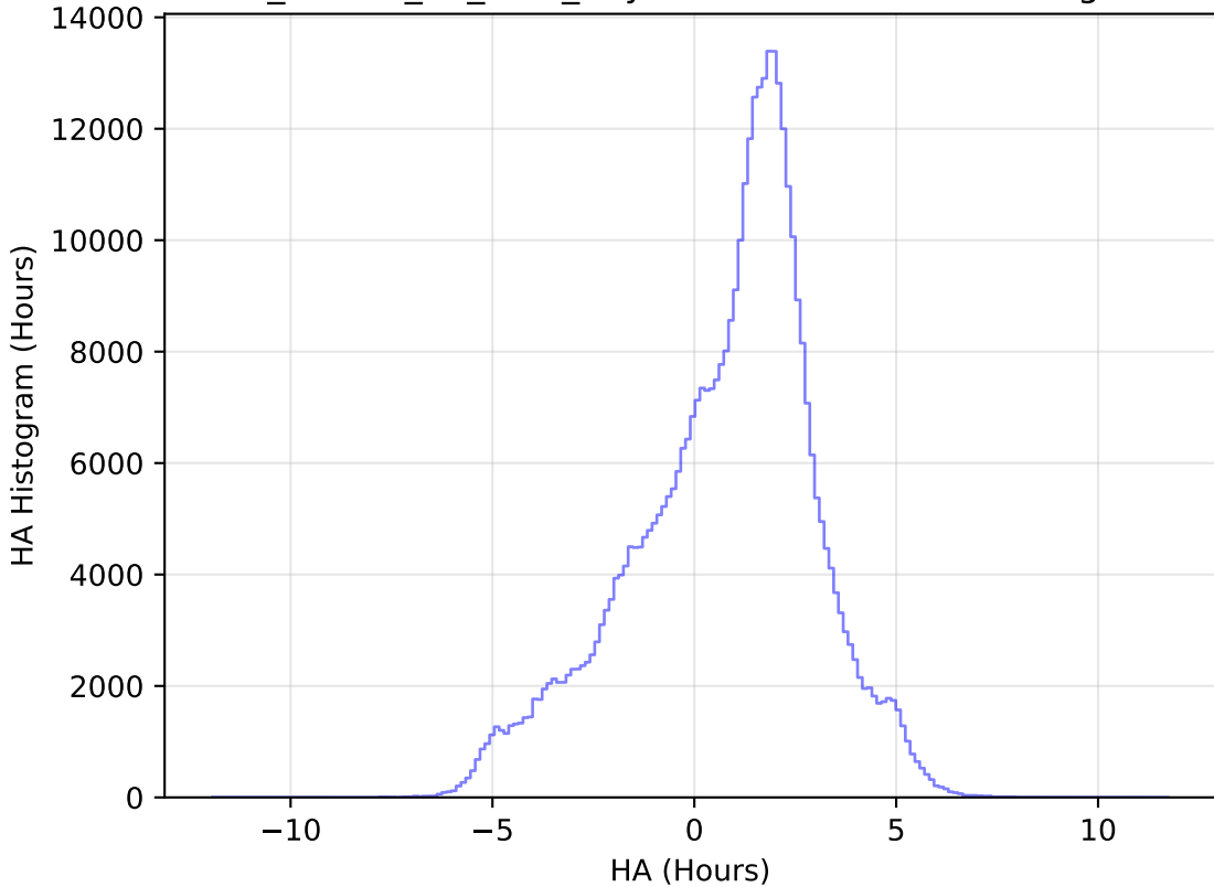
ddf_loaded_fl2_v3.4_10yrs WFD z band: HA Histogram
