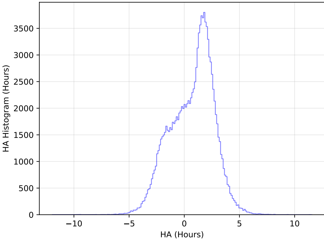
ddf_loaded_fl2_v3.4_10yrs WFD u band: HA Histogram
