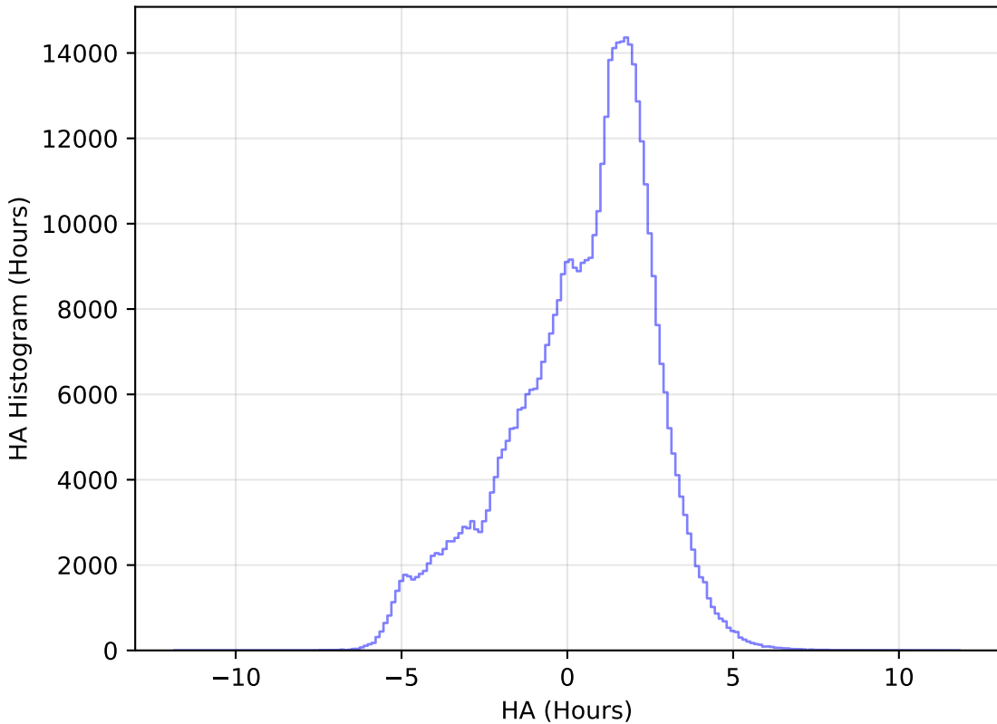
ddf_loaded_fl2_v3.4_10yrs WFD r band: HA Histogram
