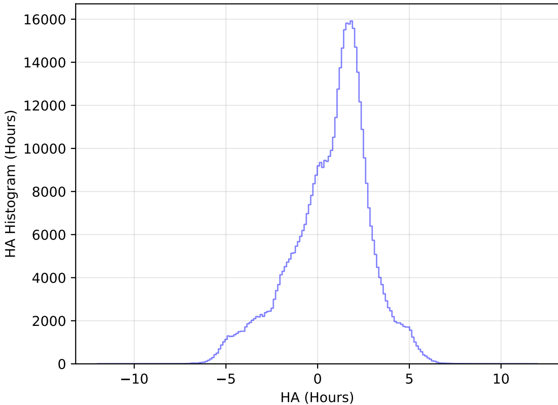
ddf_loaded_fl2_v3.4_10yrs WFD i band: HA Histogram
