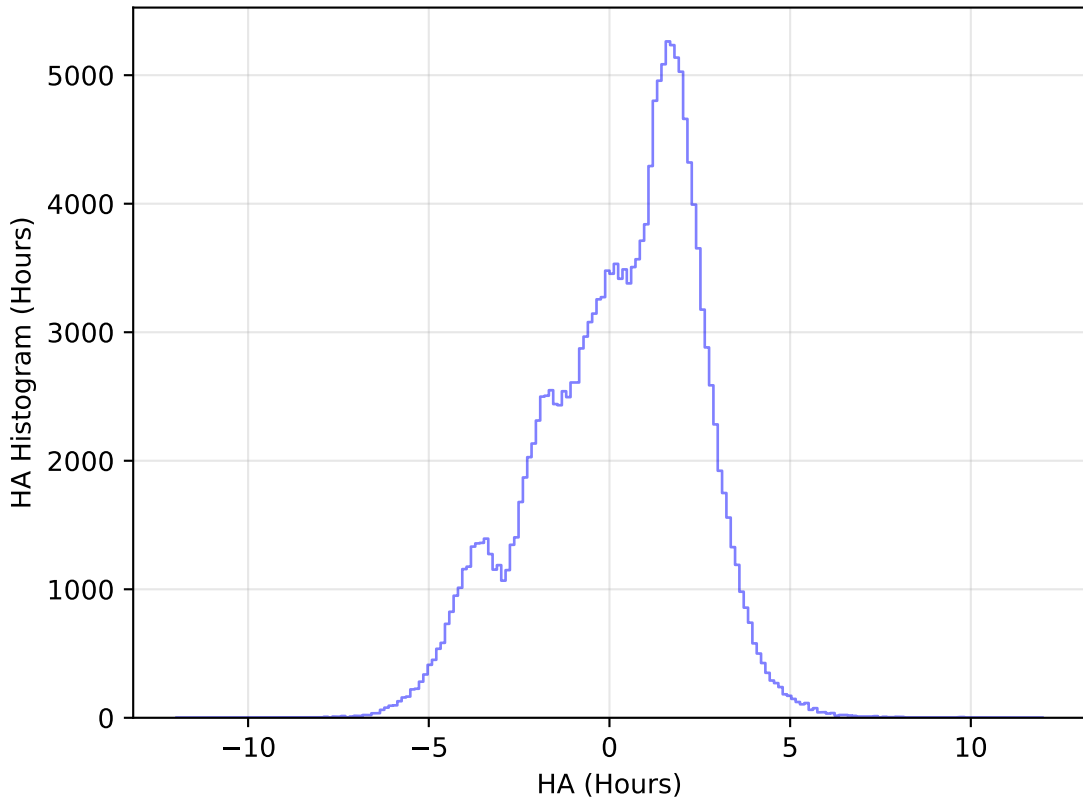
ddf_loaded_fl2_v3.4_10yrs WFD g band: HA Histogram
