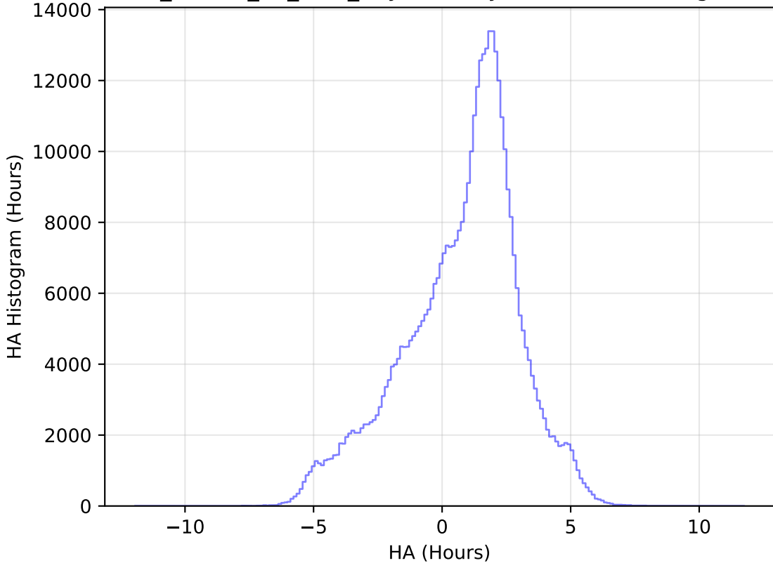
ddf_loaded_fl2_v3.4_10yrs All sky z band: HA Histogram
