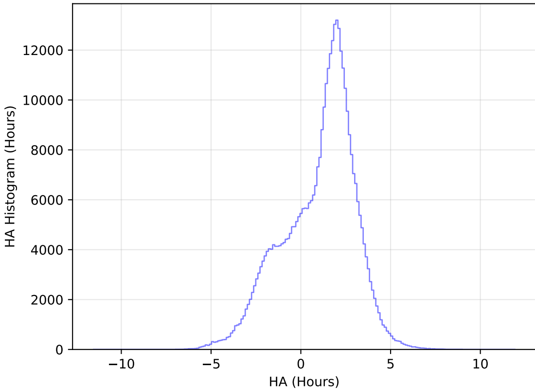
ddf_loaded_fl2_v3.4_10yrs All sky y band: HA Histogram
