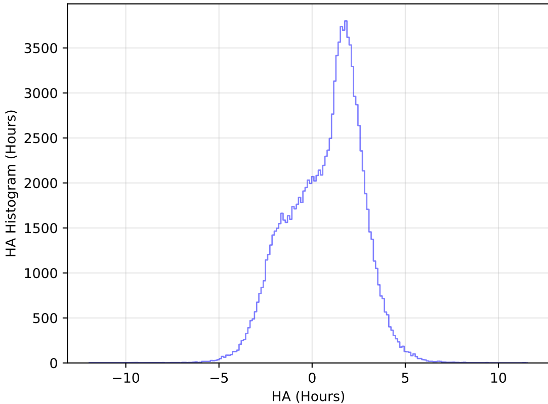
ddf_loaded_fl2_v3.4_10yrs All sky u band: HA Histogram
