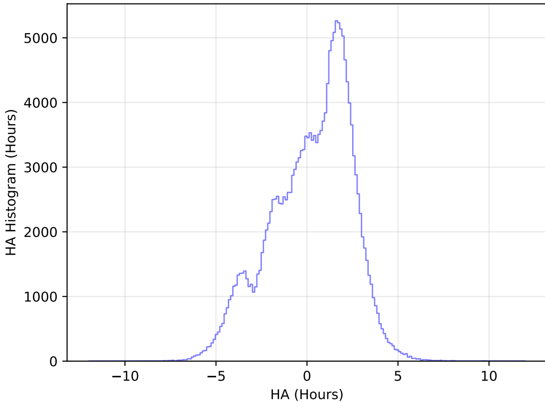
ddf_loaded_fl2_v3.4_10yrs All sky g band: HA Histogram
