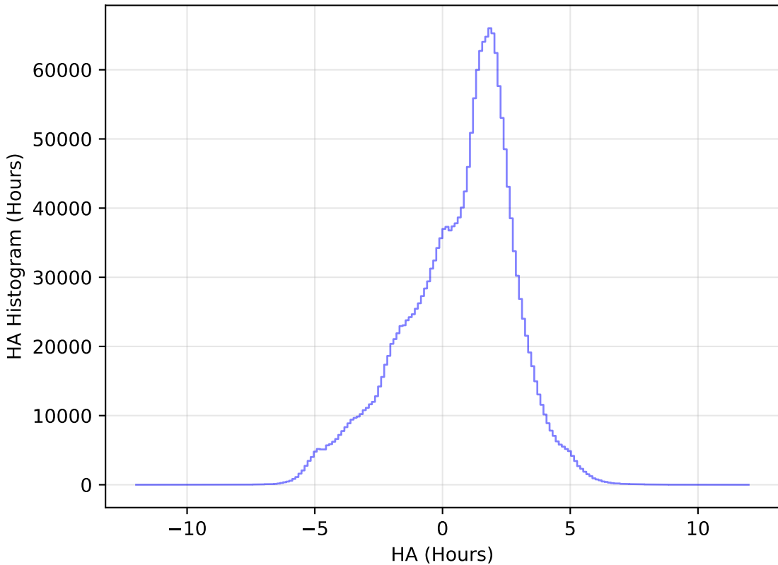
ddf_loaded_fl2_v3.4_10yrs All sky all bands: HA Histogram
