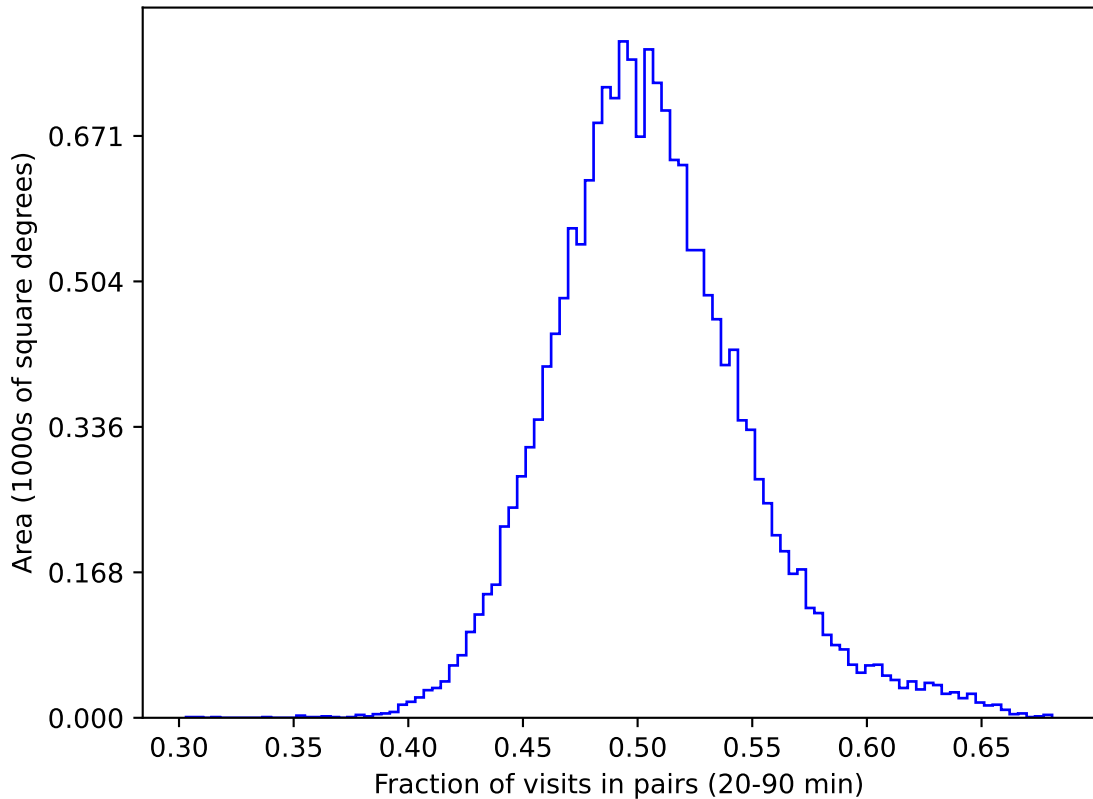
ddf_loaded_fl2_v3.4_10yrs gri WFD: Fraction of visits in pairs (20-90 min)
