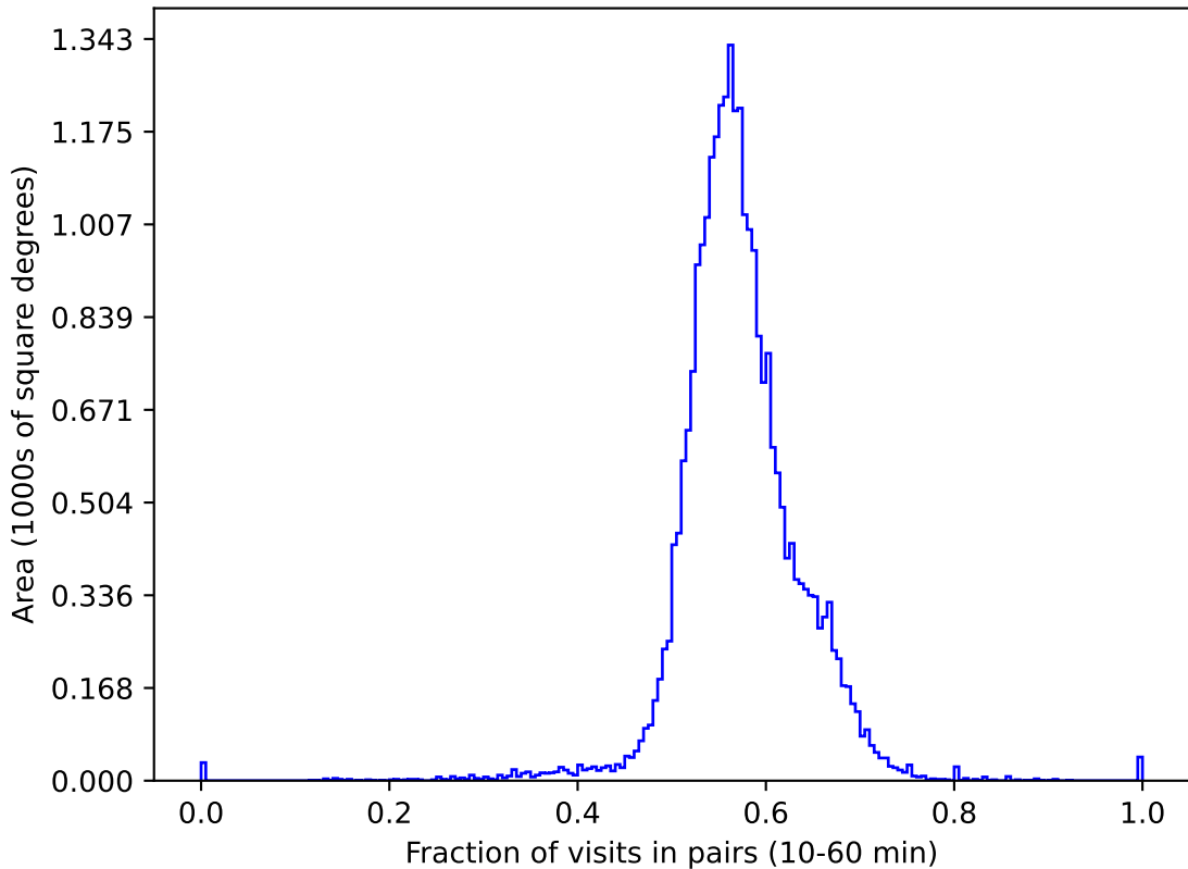
ddf_loaded_fl2_v3.4_10yrs gri All sky: Fraction of visits in pairs (10-60 min)
