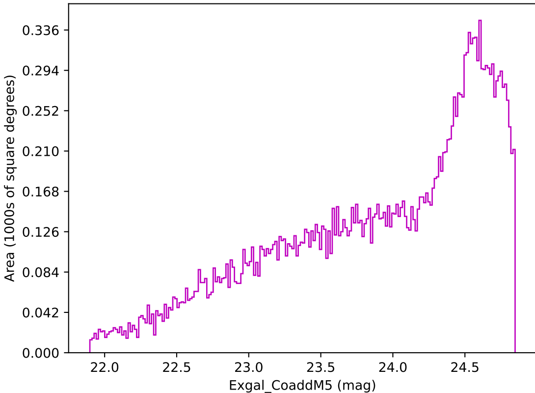
ddf_loaded_fl2_v3.4_10yrs Yr 3-4 z band: Exgal_CoaddM5
