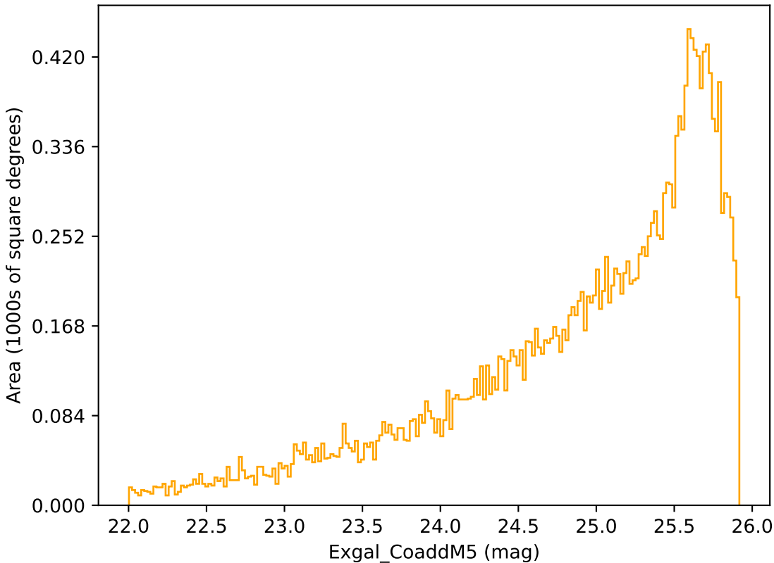
ddf_loaded_fl2_v3.4_10yrs Yr 3-4 r band: Exgal_CoaddM5
