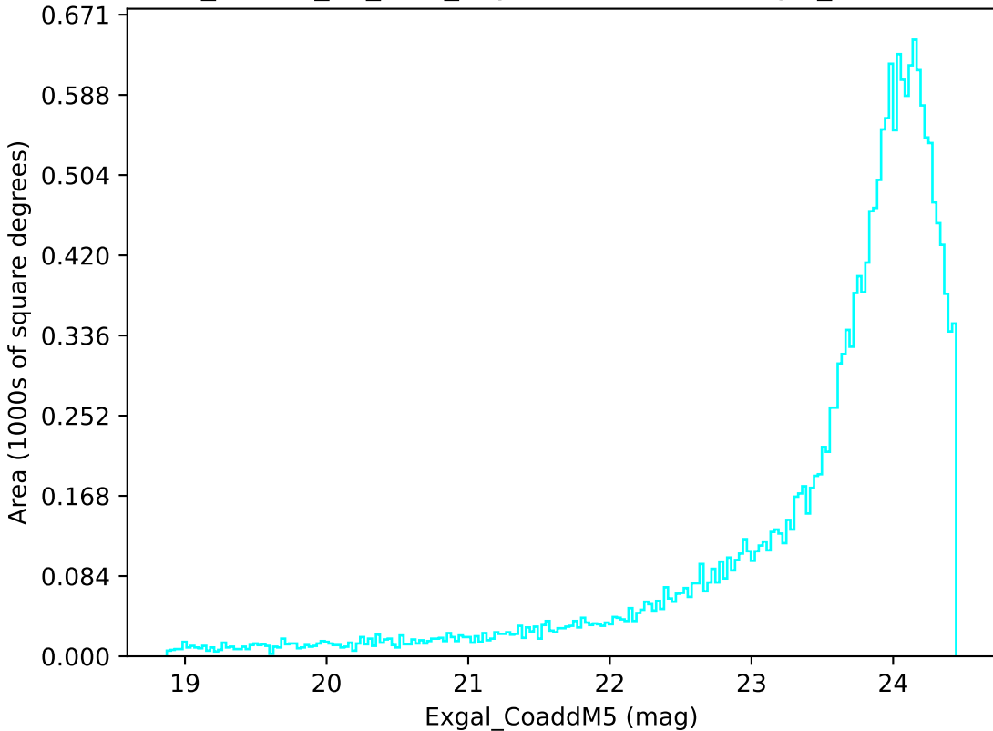
ddf_loaded_fl2_v3.4_10yrs Yr 1 u band: Exgal_CoaddM5
