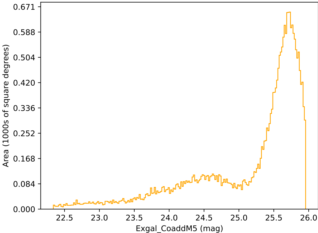
ddf_loaded_fl2_v3.4_10yrs Yr 1 r band: Exgal_CoaddM5
