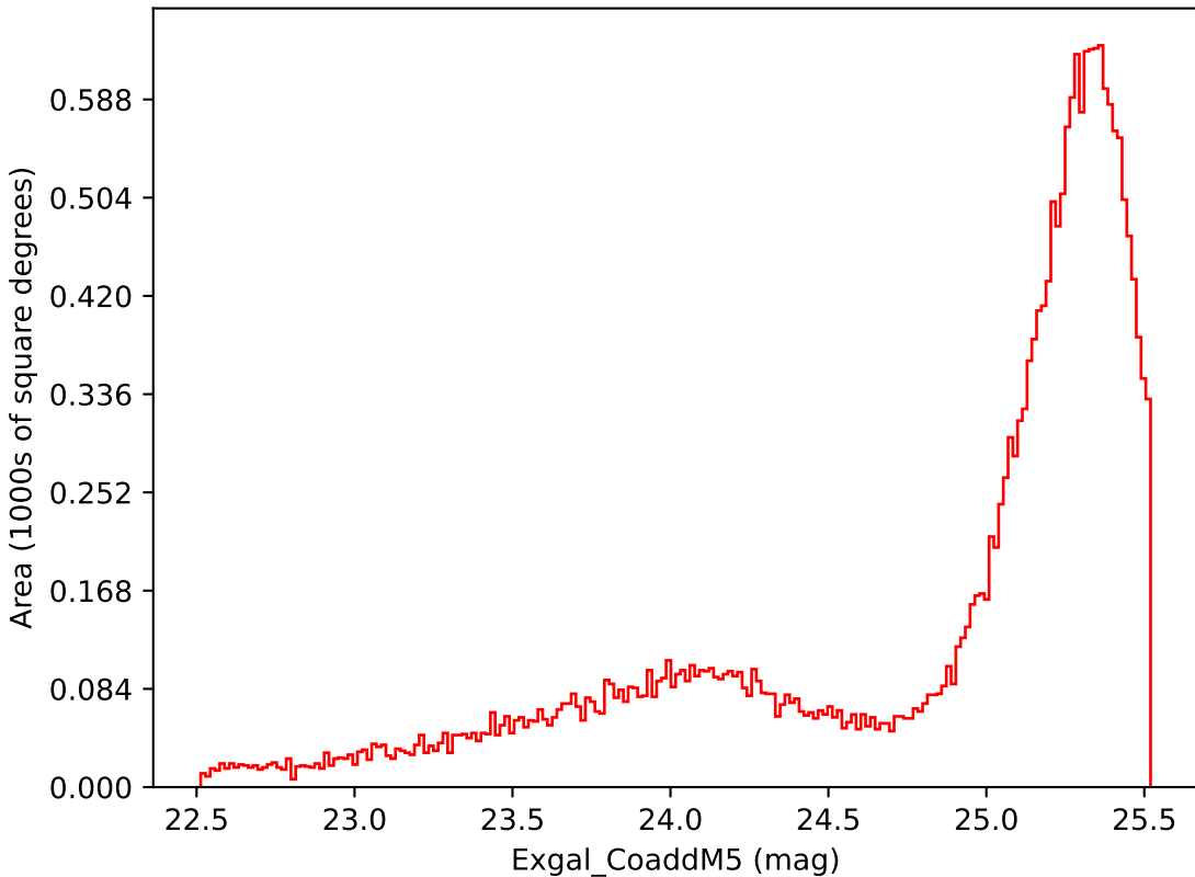
ddf_loaded_fl2_v3.4_10yrs Yr 1 i band: Exgal_CoaddM5
