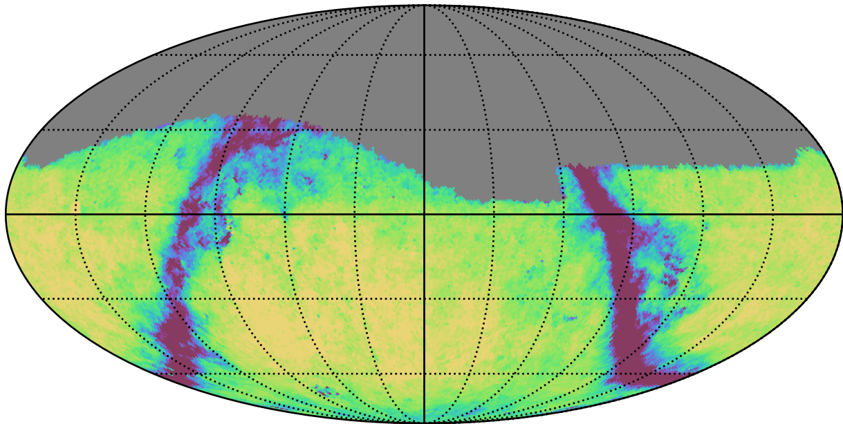
ddf_loaded_fl2_v3.4_10yrs Yr 1 g band: Exgal_CoaddM5
