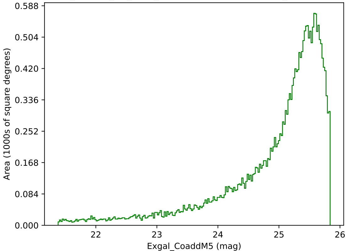
ddf_loaded_fl2_v3.4_10yrs Yr 1 g band: Exgal_CoaddM5
