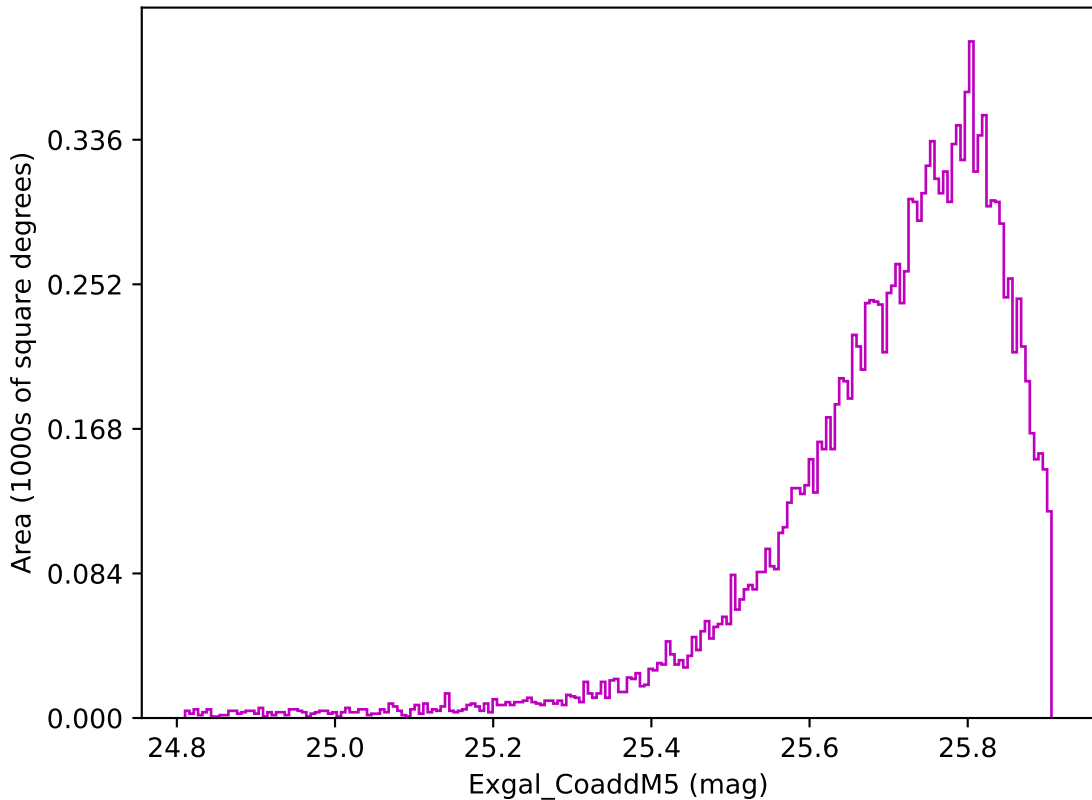
ddf_loaded_fl2_v3.4_10yrs WFD z band: Exgal_CoaddM5
