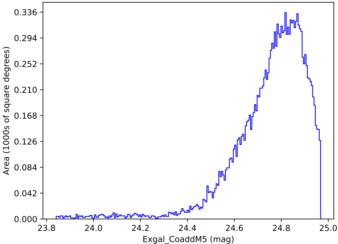
ddf_loaded_fl2_v3.4_10yrs WFD y band: Exgal_CoaddM5
