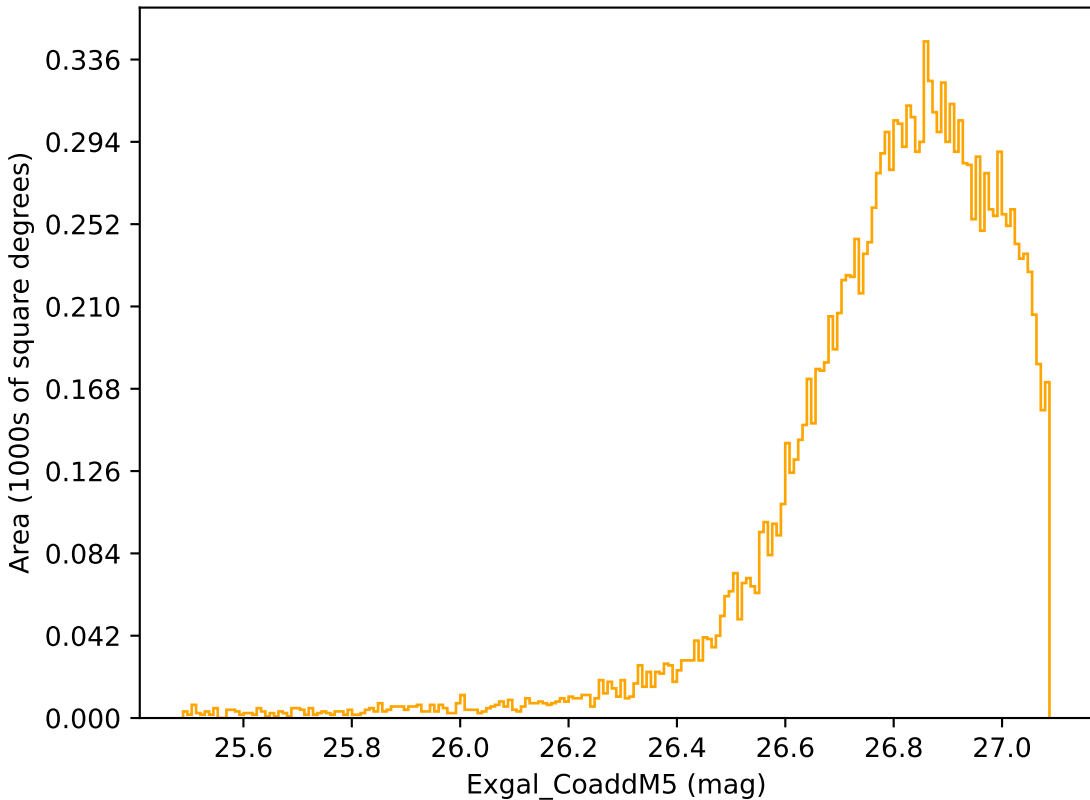
ddf_loaded_fl2_v3.4_10yrs WFD r band: Exgal_CoaddM5
