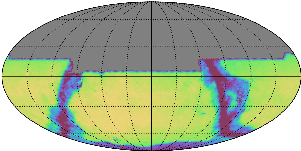
ddf_loaded_fl2_v3.4_10yrs All sky y band: Exgal_CoaddM5
