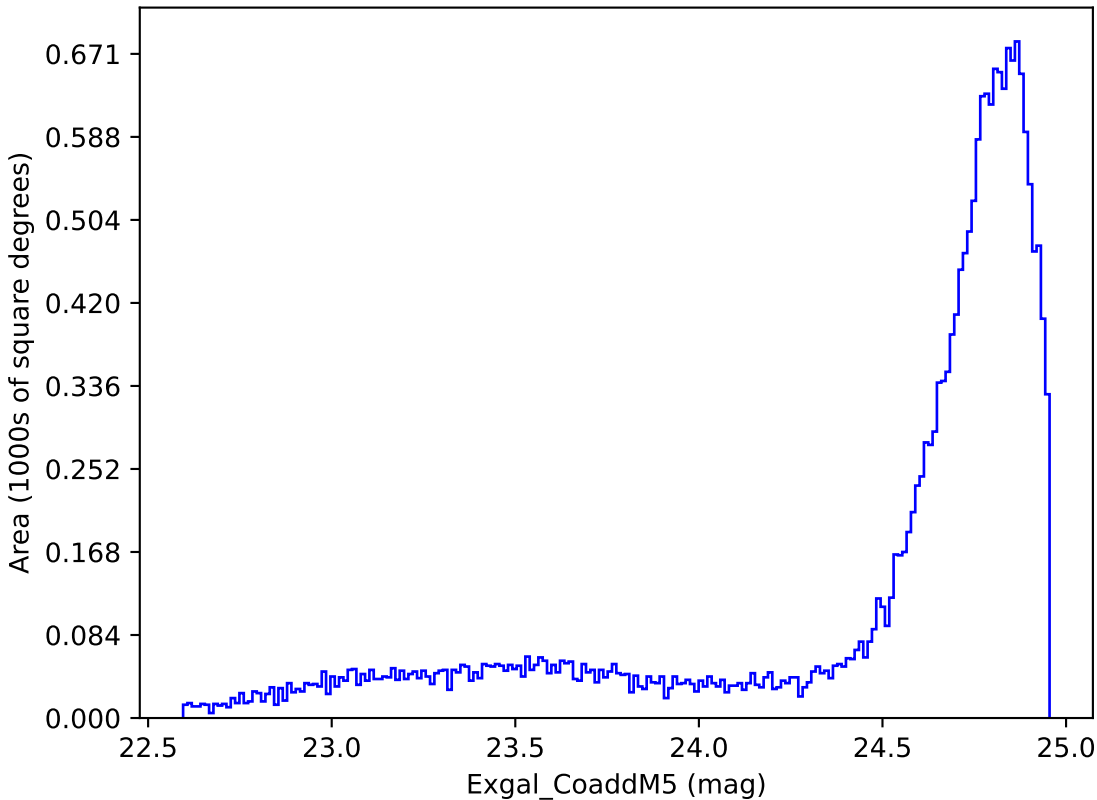
ddf_loaded_fl2_v3.4_10yrs All sky y band: Exgal_CoaddM5
