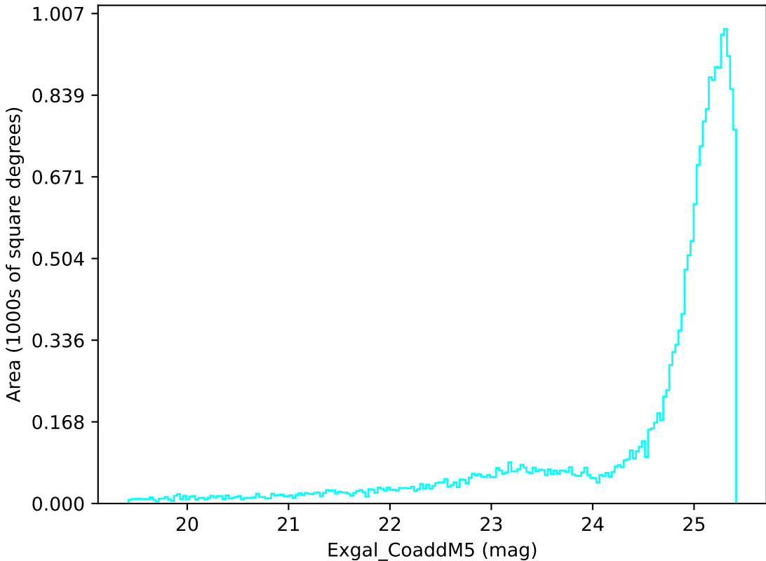
ddf_loaded_fl2_v3.4_10yrs All sky u band: Exgal_CoaddM5
