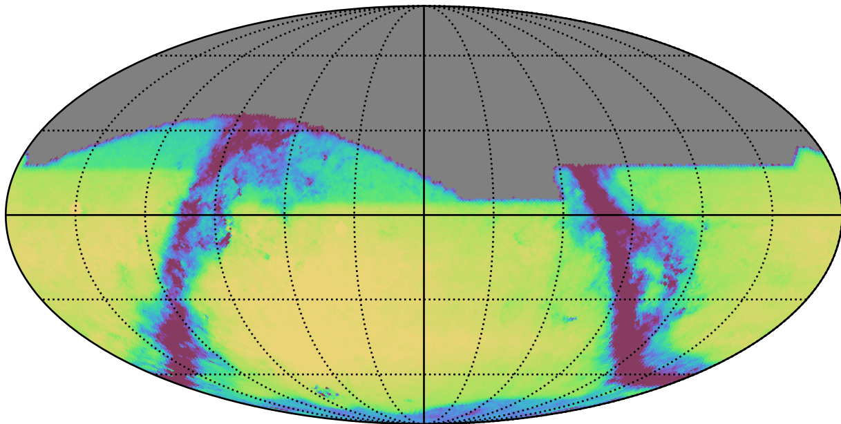
ddf_loaded_fl2_v3.4_10yrs All sky r band: Exgal_CoaddM5
