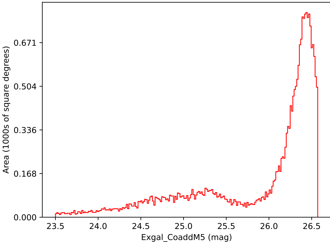
ddf_loaded_fl2_v3.4_10yrs All sky i band: Exgal_CoaddM5
